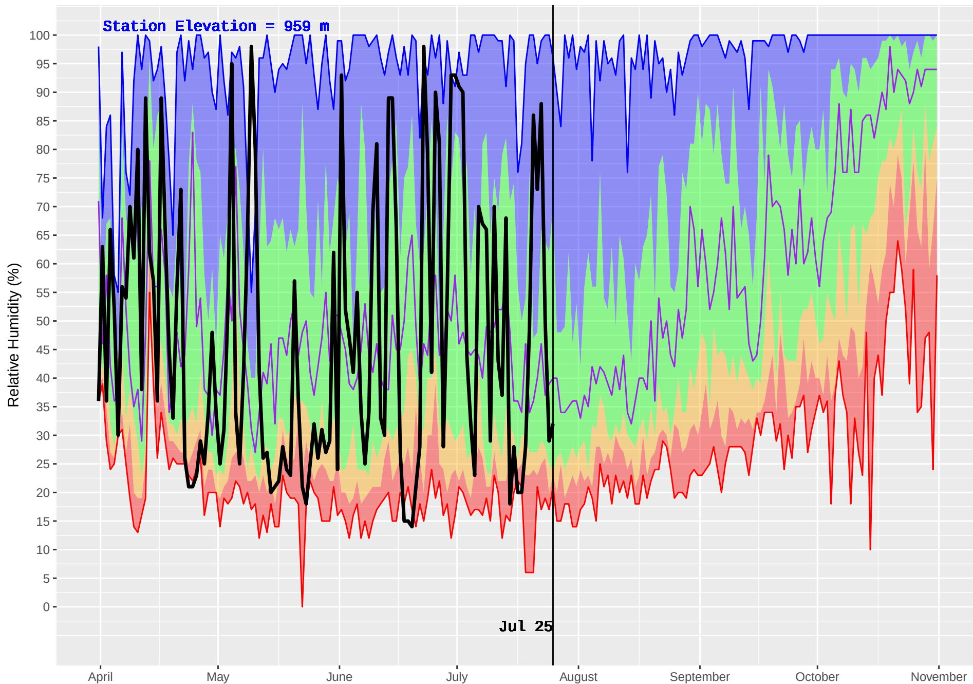
WELLS GRAY (266) : Historical (1994–2016) and Current (2018) Noon Relative Humidity
