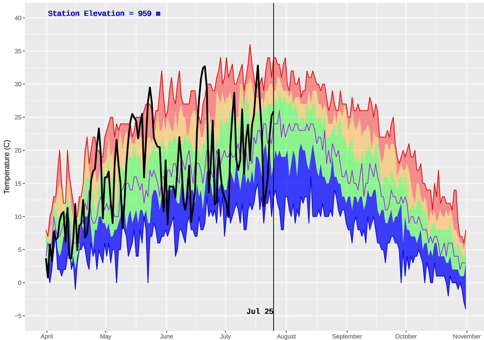
WELLS GRAY (266) : Historical (1994–2016) and Current (2018) Noon Temperature
