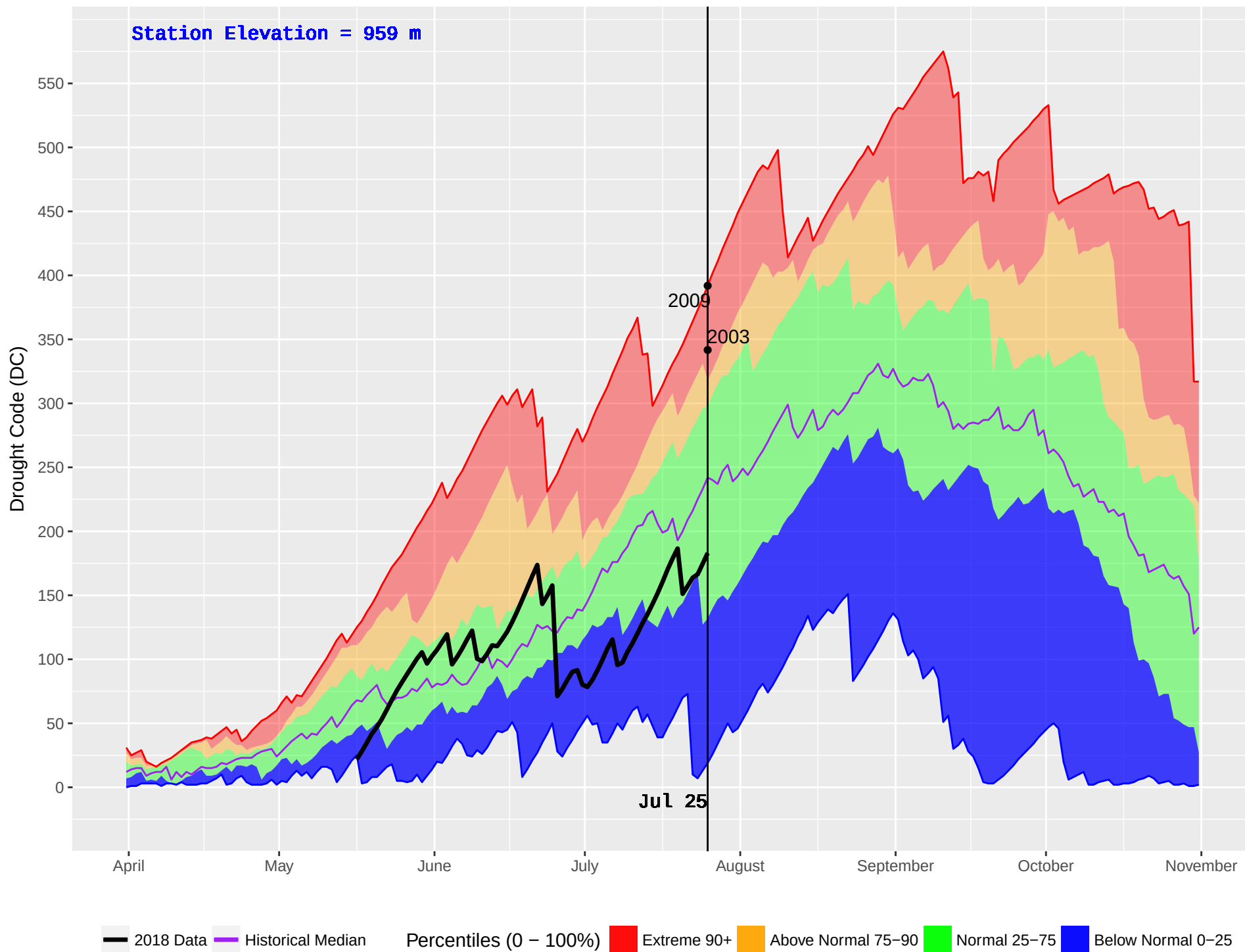
WELLS GRAY (266) : Historical (1994–2016) and Current (2018) Noon Drought Code (DC)
