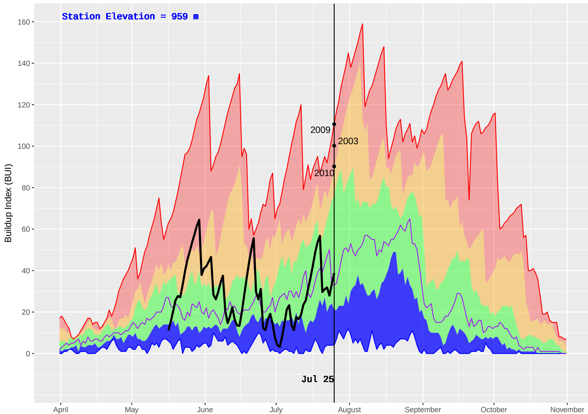
WELLS GRAY (266) : Historical (1994–2016) and Current (2018) Noon Buildup Index (BUI)
